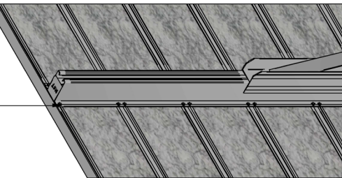
DETAIL 3 1:10
