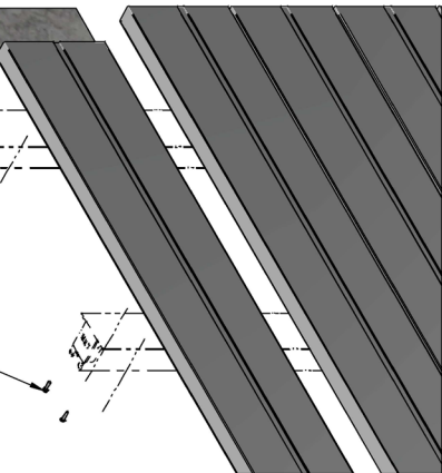
PANEL END & NON JOIN POST FIXING DETAIL
