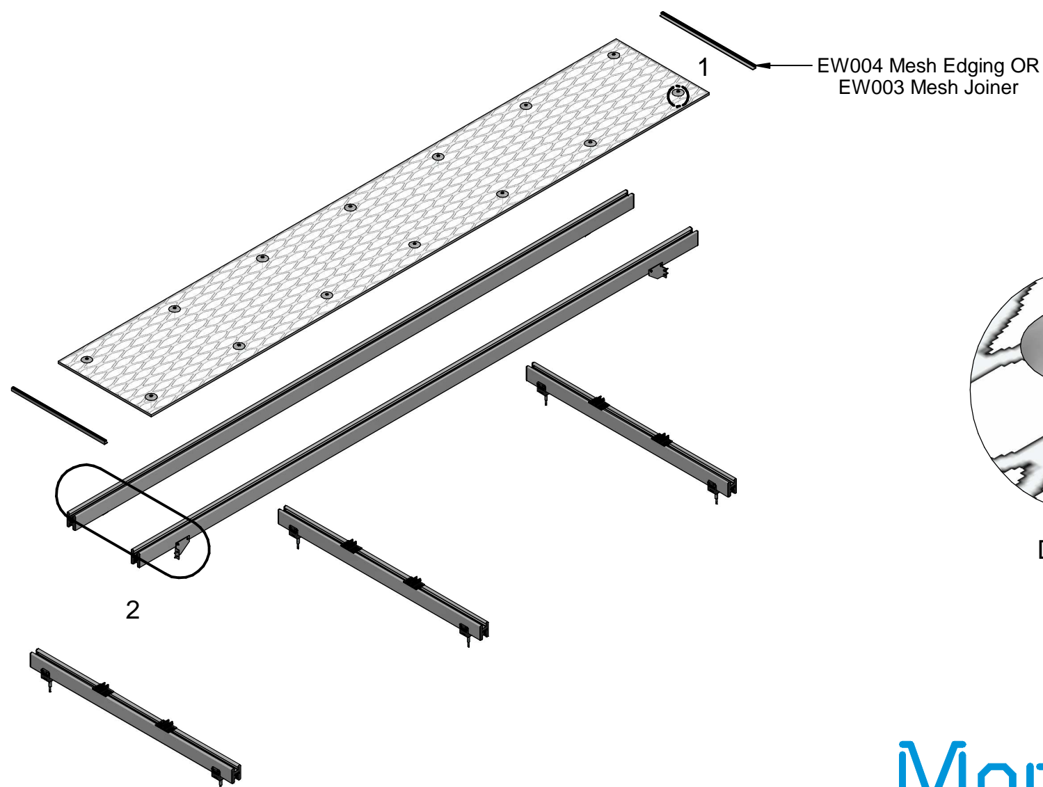
EXPLODED VIEW
