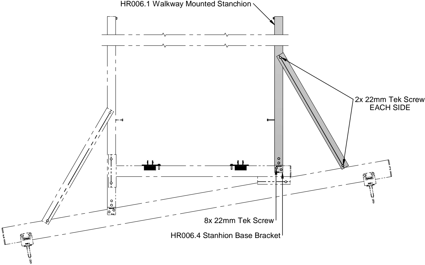
SKYWALK SUPPORT (LEVELLED WITH DOUBLE HANDRAIL)
