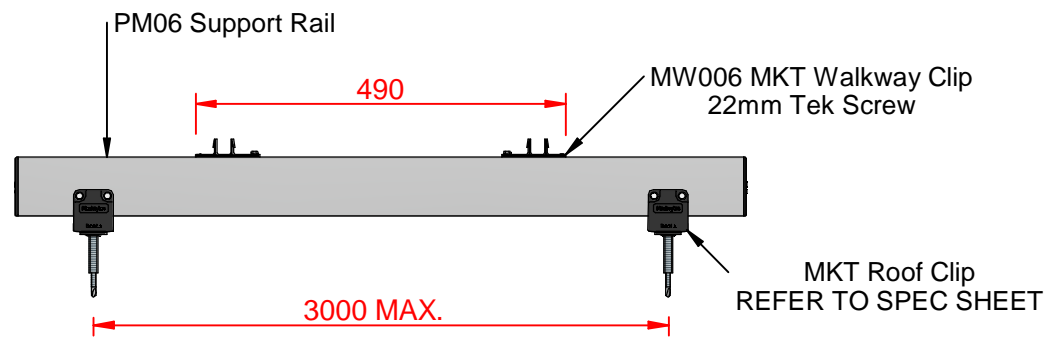
SKYWALK SUPPORT (STANDARD)
