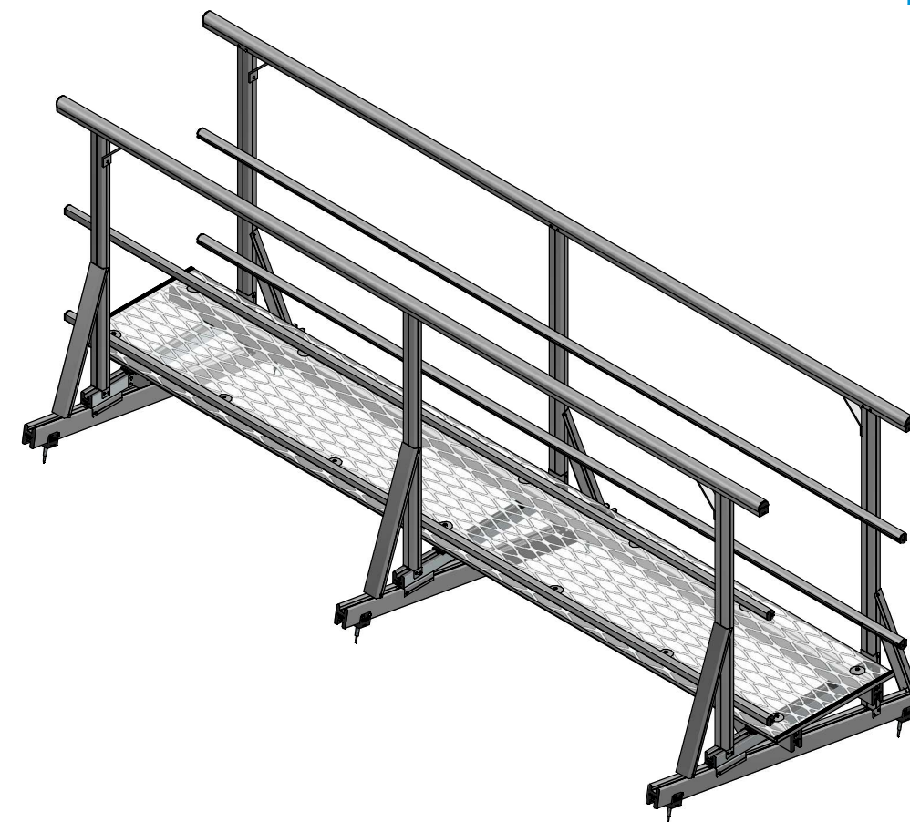
SKYWALK WITH MESH (LEVELLED WITH HANDRAILS)
