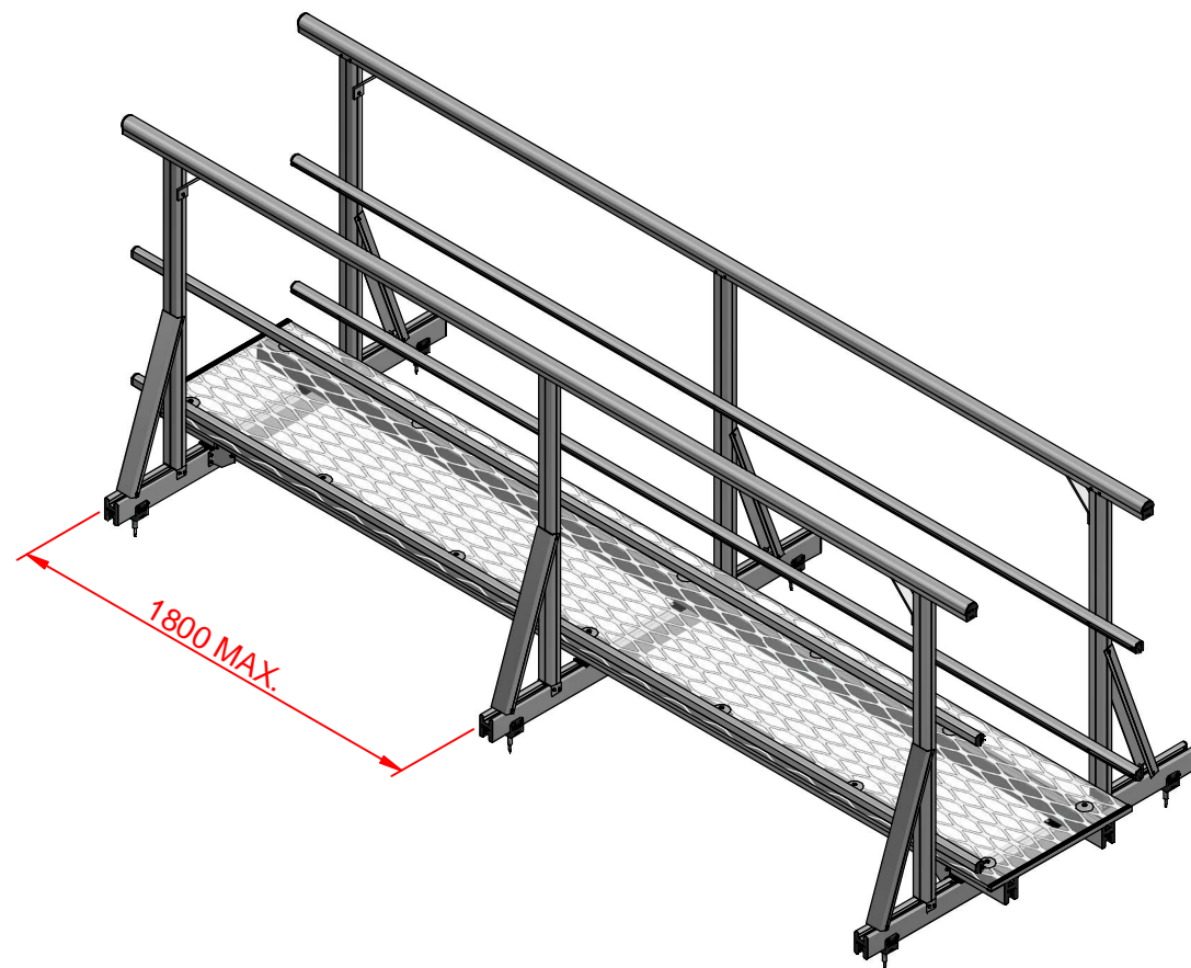
SKYWALK WITH MESH (HANDRAILS)
