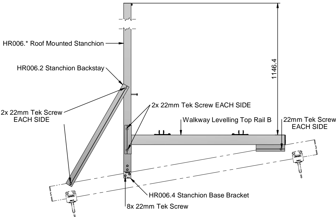
SKYWALK SUPPORT (LEVELLED WITH SINGLE HANDRAIL)
