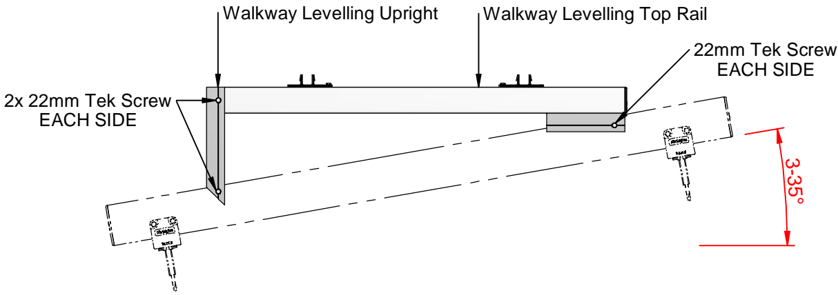
SKYWALK SUPPORT (LEVELLED)
