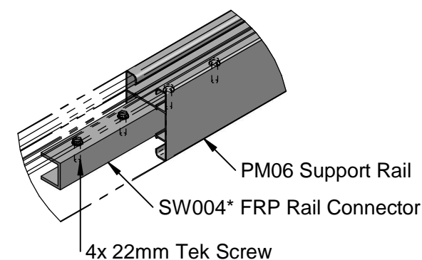
PM06 JOIN DETAIL (FOR SKYWALK OVER 6000mm) 1:5
