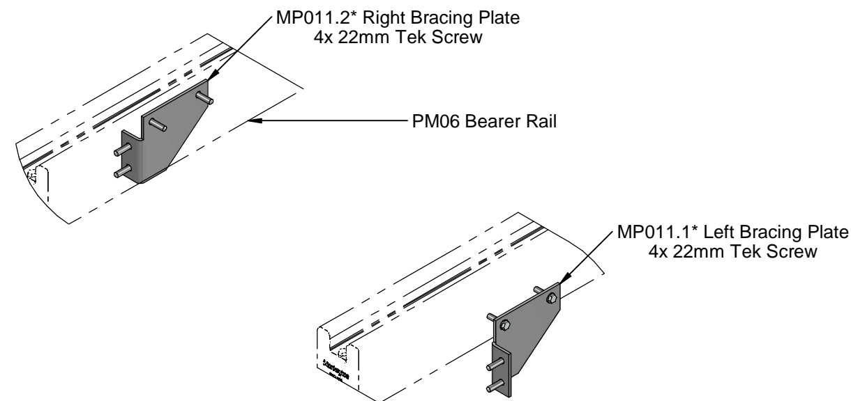
DETAIL 2 1:5
