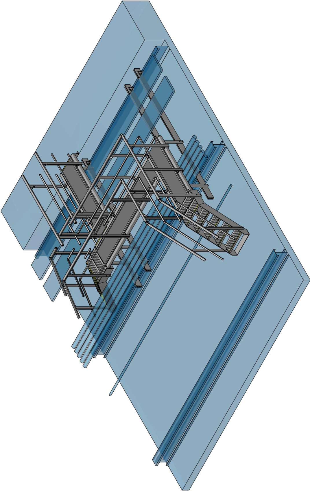
ISOMETRIC VIEW 1:35
