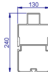
PM45 USAGE: Acoustic Screens LENGTH: 4800mm
