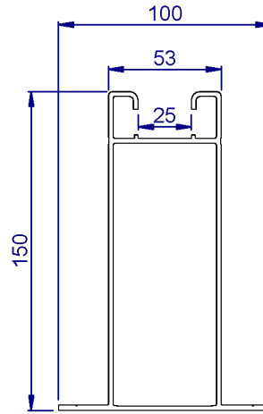
PM34 USAGE: Screen Support/Heavy Duty Rail LENGTH: 5800mm
