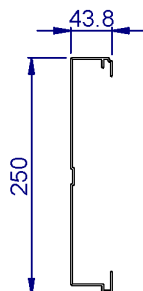
PM51 USAGE: Hushmonkey Acoustic Panel LENGTH: 4810mm
