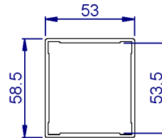
PM38 USAGE: Truss Member, Joiner For MKT Extrusions LENGTH: 6000mm
