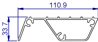
PM28 USAGE: Stepladder Tread LENGTH: 5000mm
