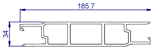
PM41 USAGE: X-Beam Web Section LENGTH: 11000mm
