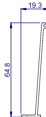
PM43 USAGE: X-Beam Cap LENGTH: 11000mm
