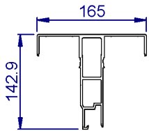
PM40 USAGE: X-Beam Flange LENGTH: 11000mm
