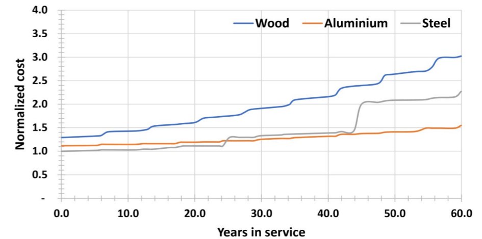
Figure 5: Life Cycle Cost Assessment of 30m Wood, Aluminium and Steel Pedestrian Bridge [2]
